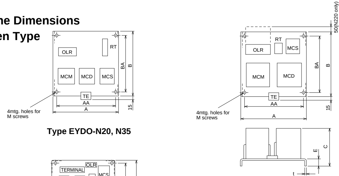
Type EYDO-N50~N220
